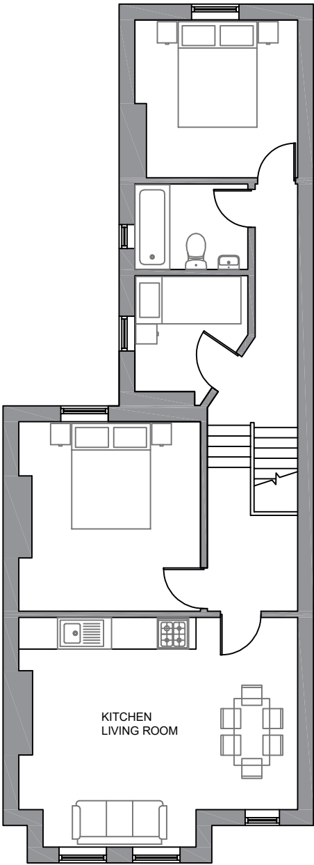
FIRST FLOOR
